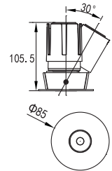
PL-MD45R-15W
